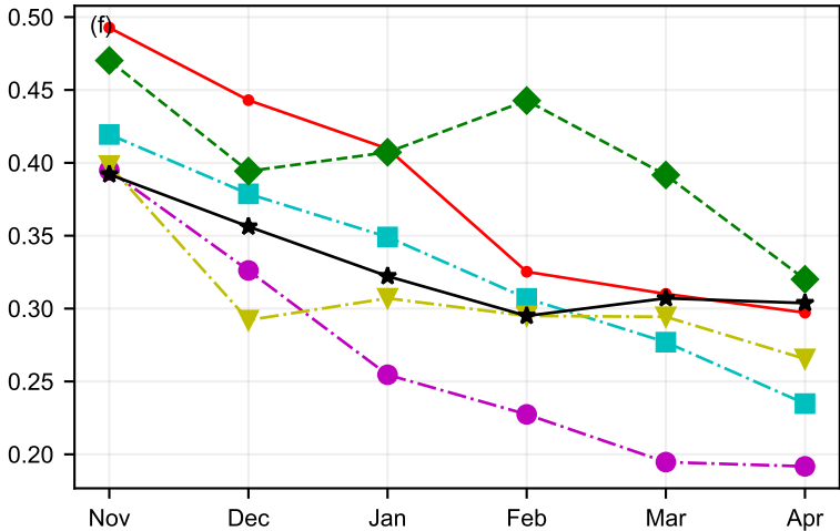
Multi-year ice fraction
